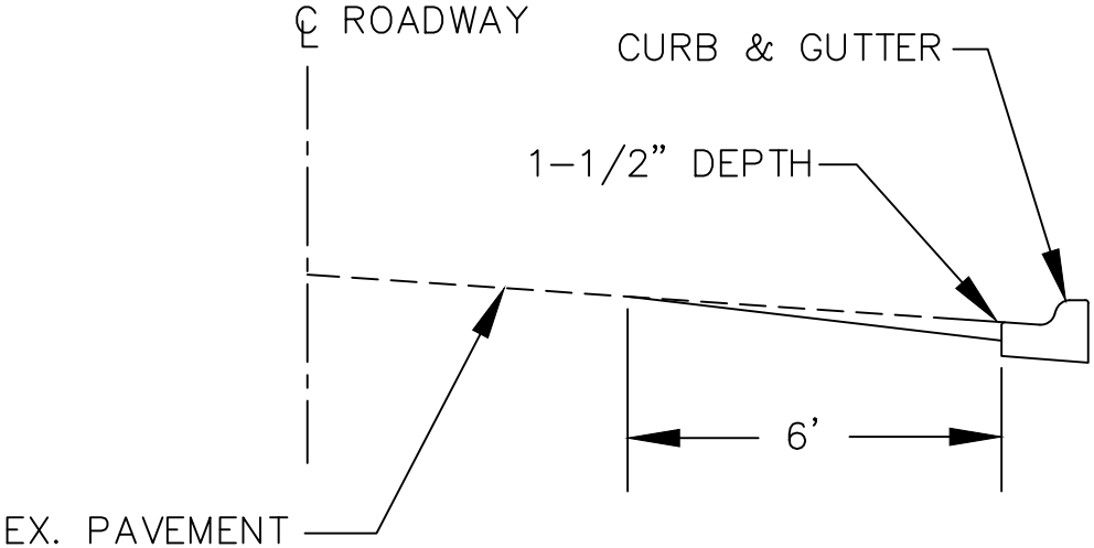
BITUMINOUS EDGE MILLING DETAIL
