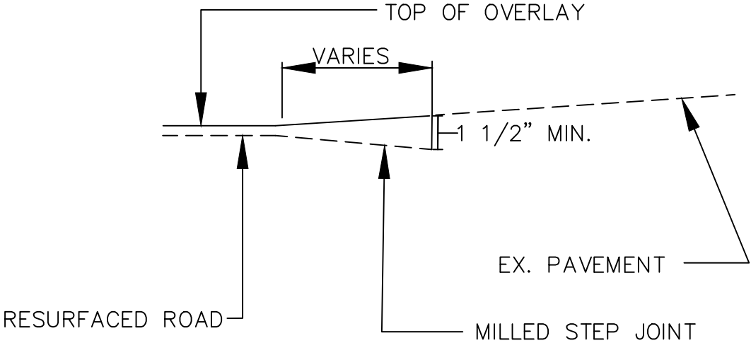
STEP JOINT DETAIL
