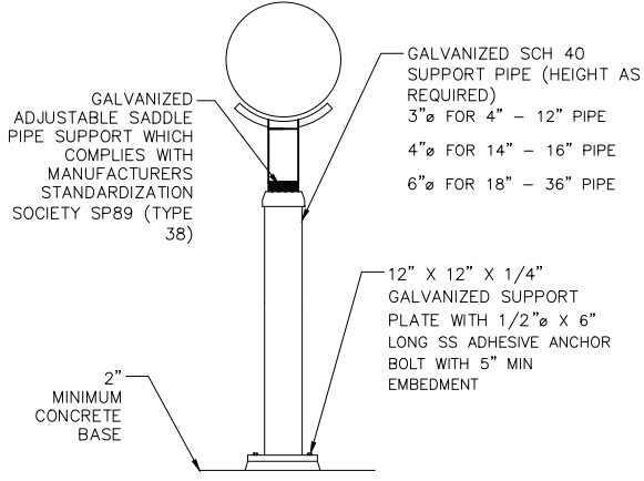
① PIPE SUPPORT FROM FLOOR DETAIL
