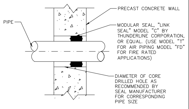
④ PIPE OPENING DETAIL
