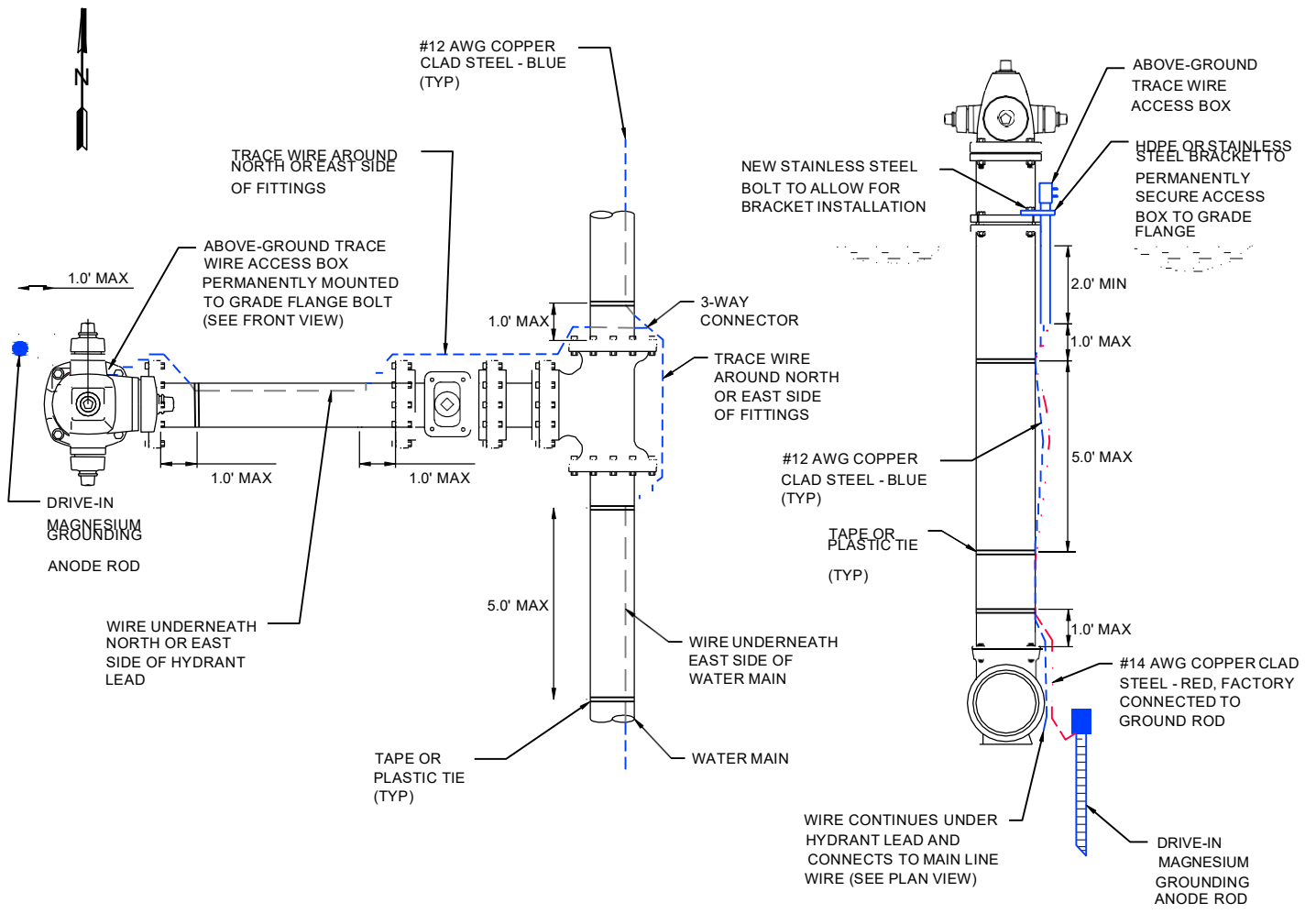
HYDRANT - PLAN VIEW NO SCALE
